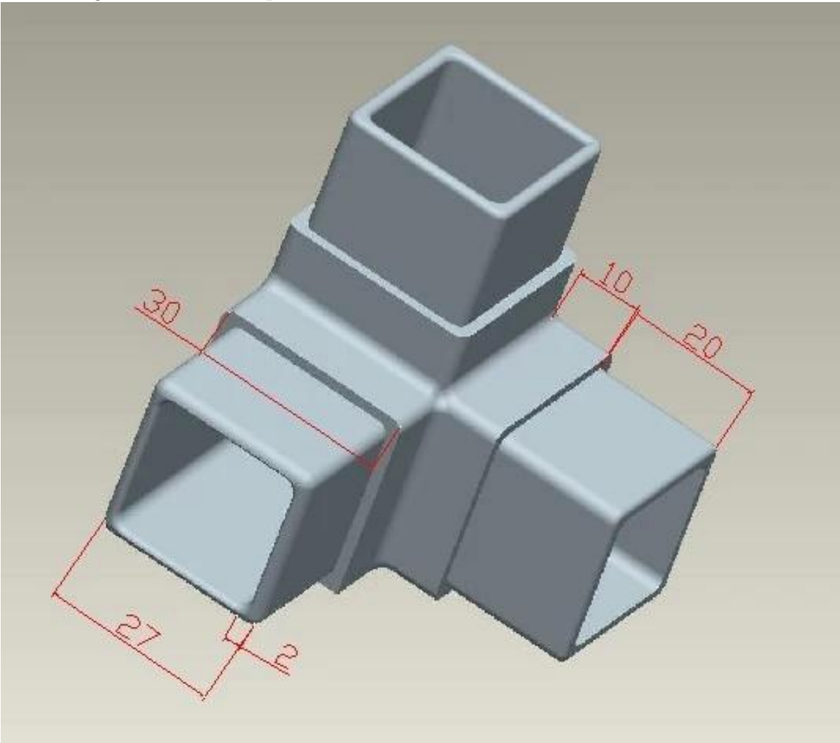
3. Drawings for 30x30mm square tube connector stainless steel
