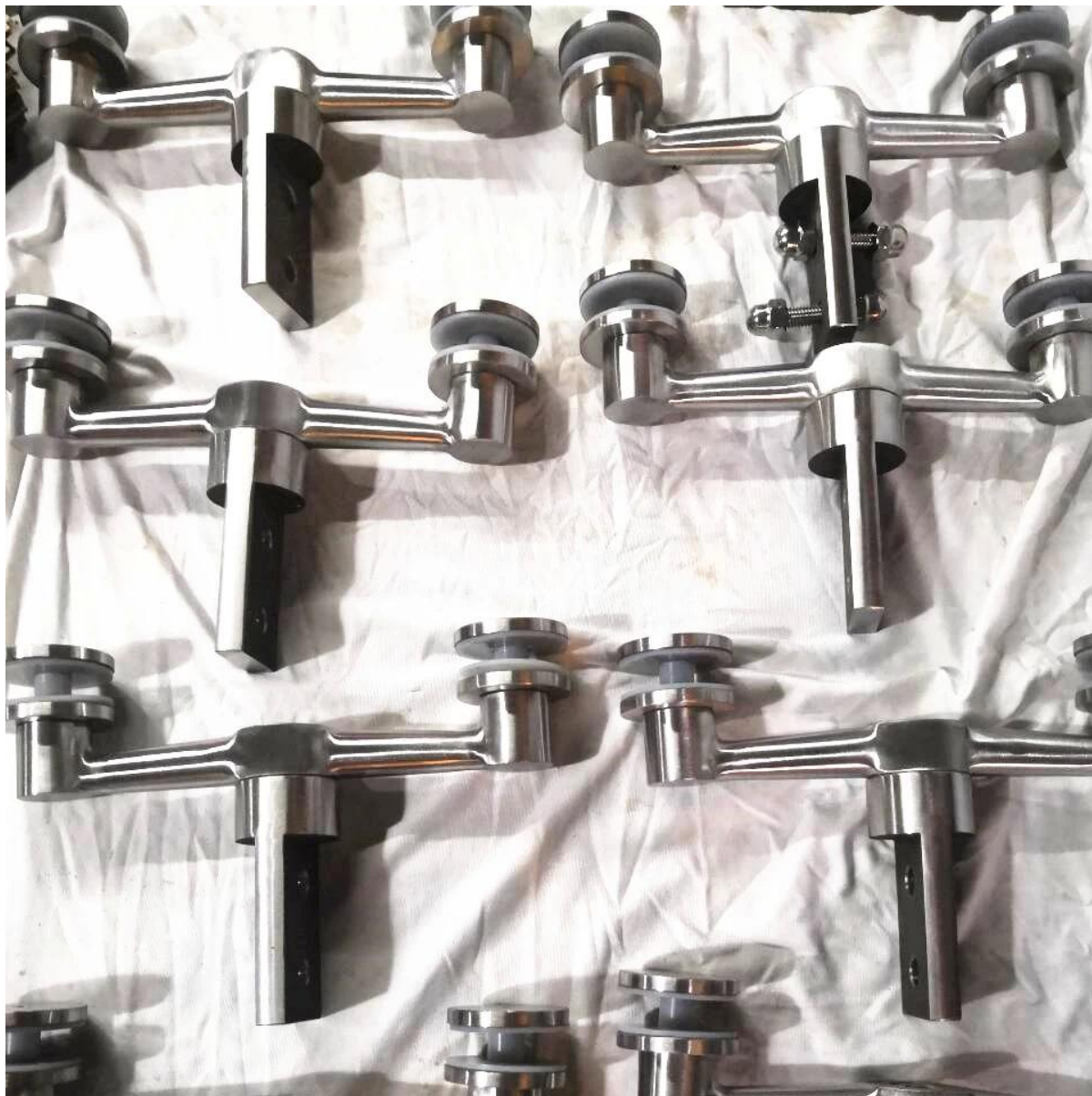
Project photo of glass spider fitting for curtain walls -
