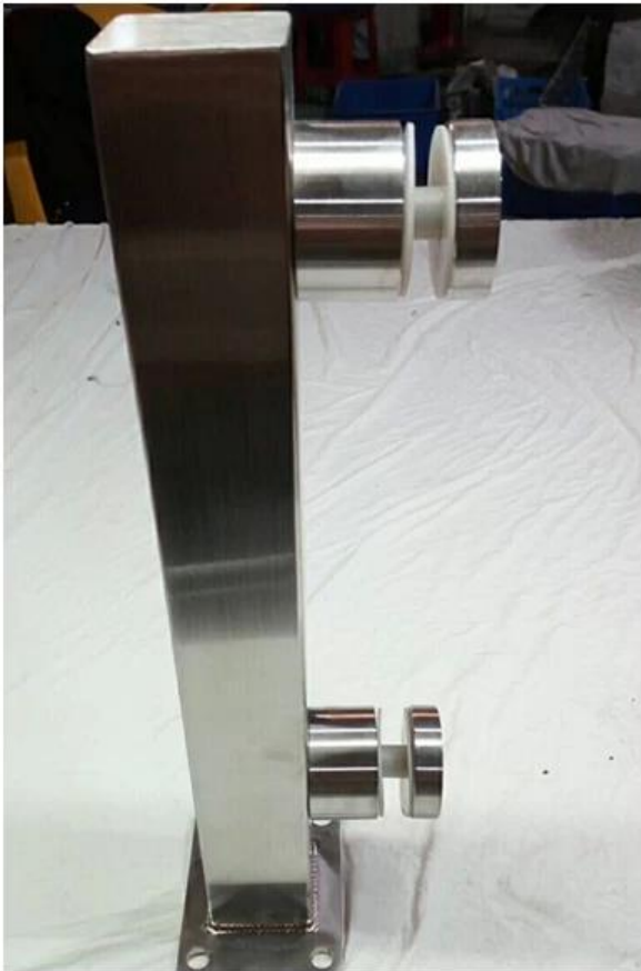
5. Stainless Steel Standoff Post & Handrail design :
