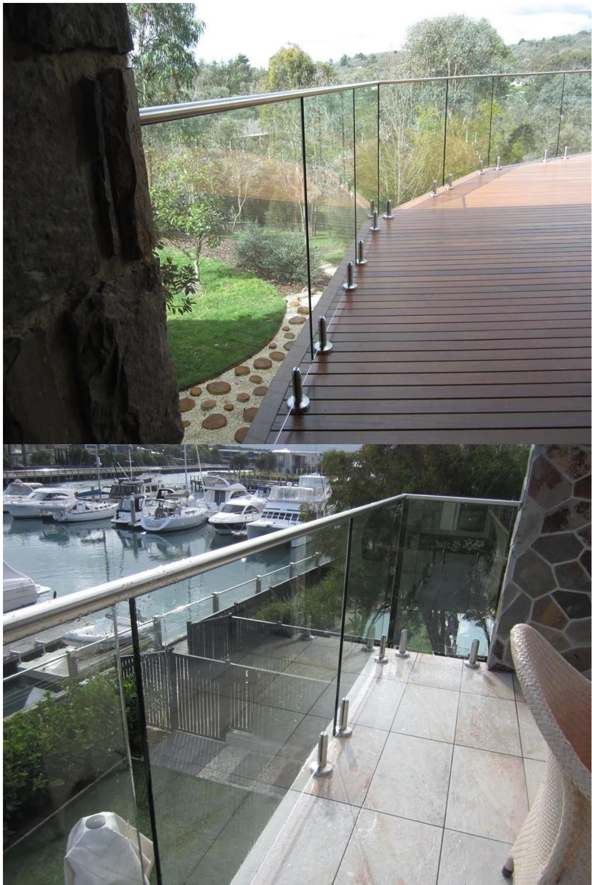
Stainless steel round handrail tube and glass standoff for outdoors handrail design
