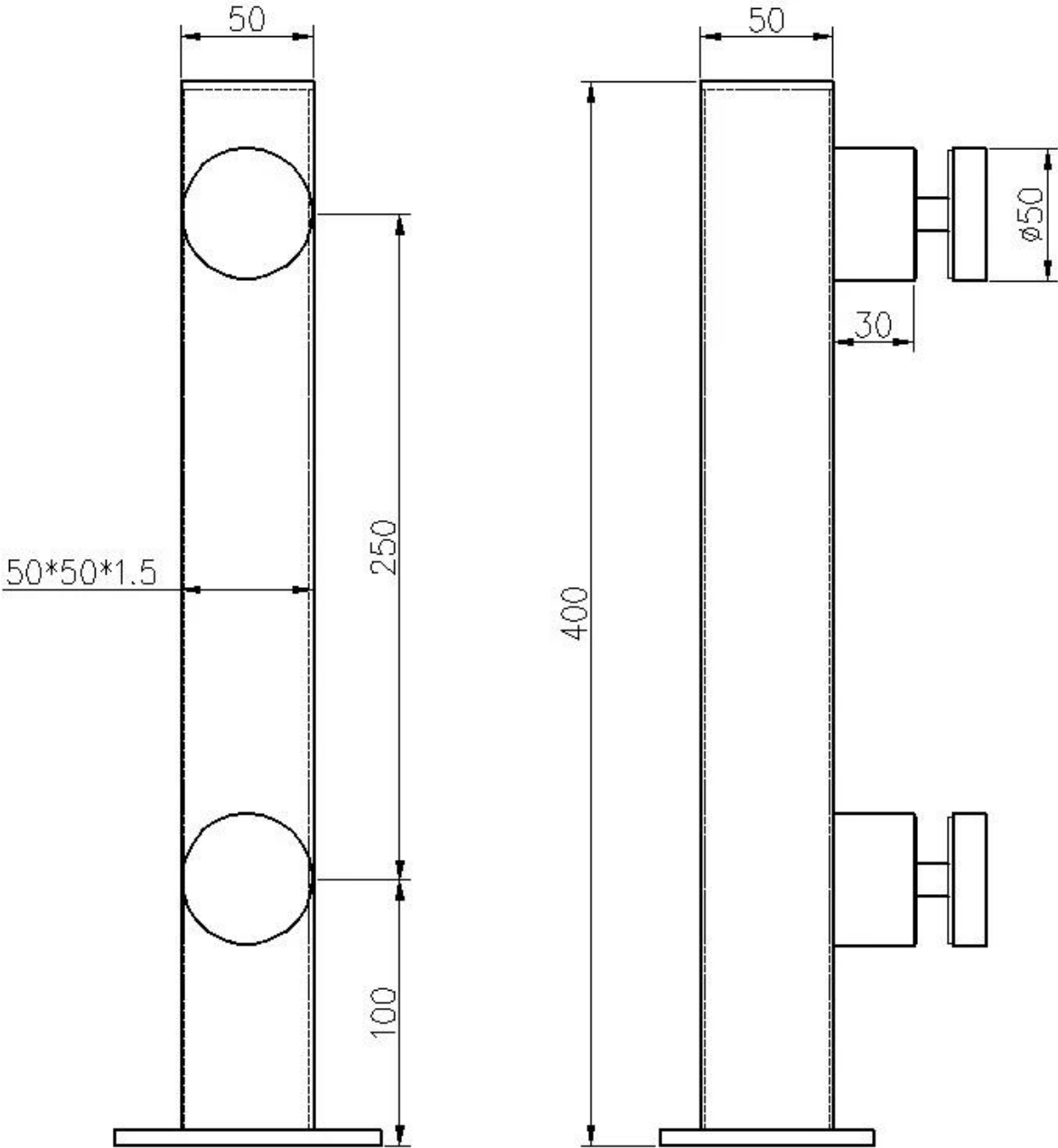
Short handrail post dimension
