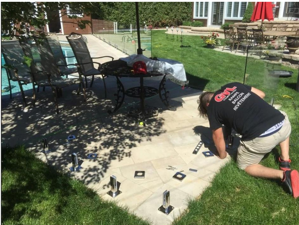
4. project photo stainless steel square glass spigot
