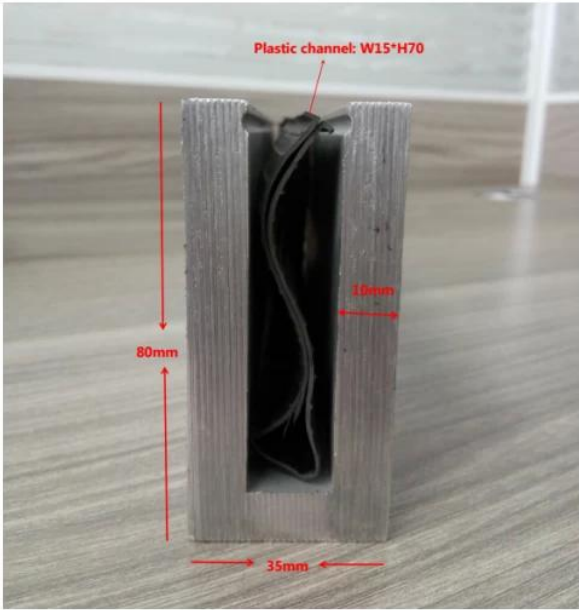
Small profile: for glass thickness 10-12.76mm
