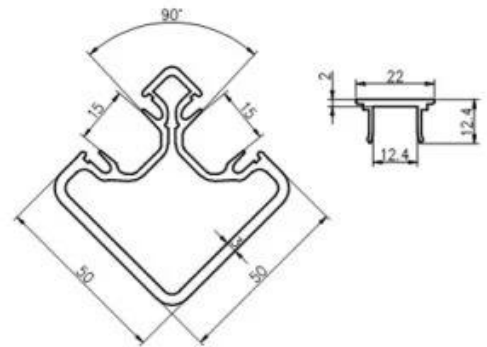
90° corner post
