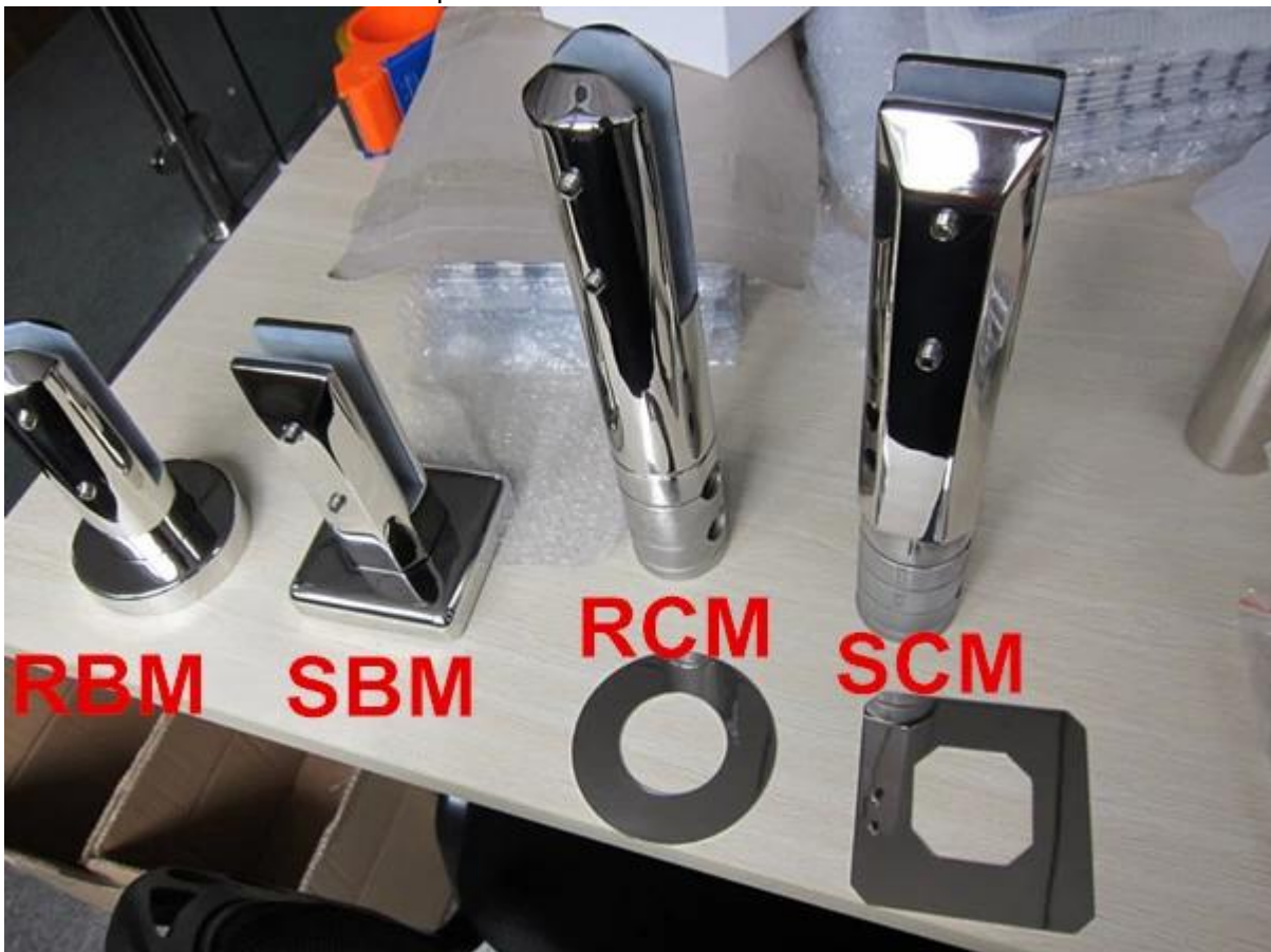
Rund Kernbohrer Pool Zaun Zapfen-Modell. RCM
