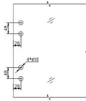
Hole dimensions
