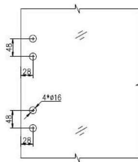
Hole dimensions
