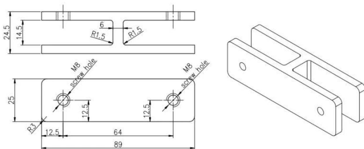
Glass TO GLASS HOLDER 180°
