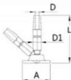
Swageless Balustrade Adjuster Flat
