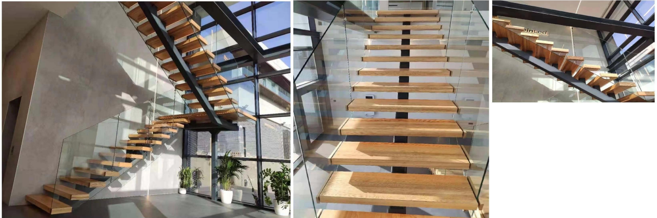
单龙骨楼梯 Single Stringer U shape stairs for Spain client 玻璃护栏 Glass handrail 镜钉护栏 Standoff glass railing with wood cover
