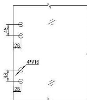
Hole dimensions
