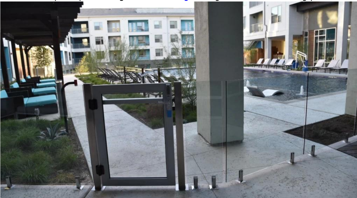
80x80mm square post and glass latch , hinge design for safe swimming pool fence gate
