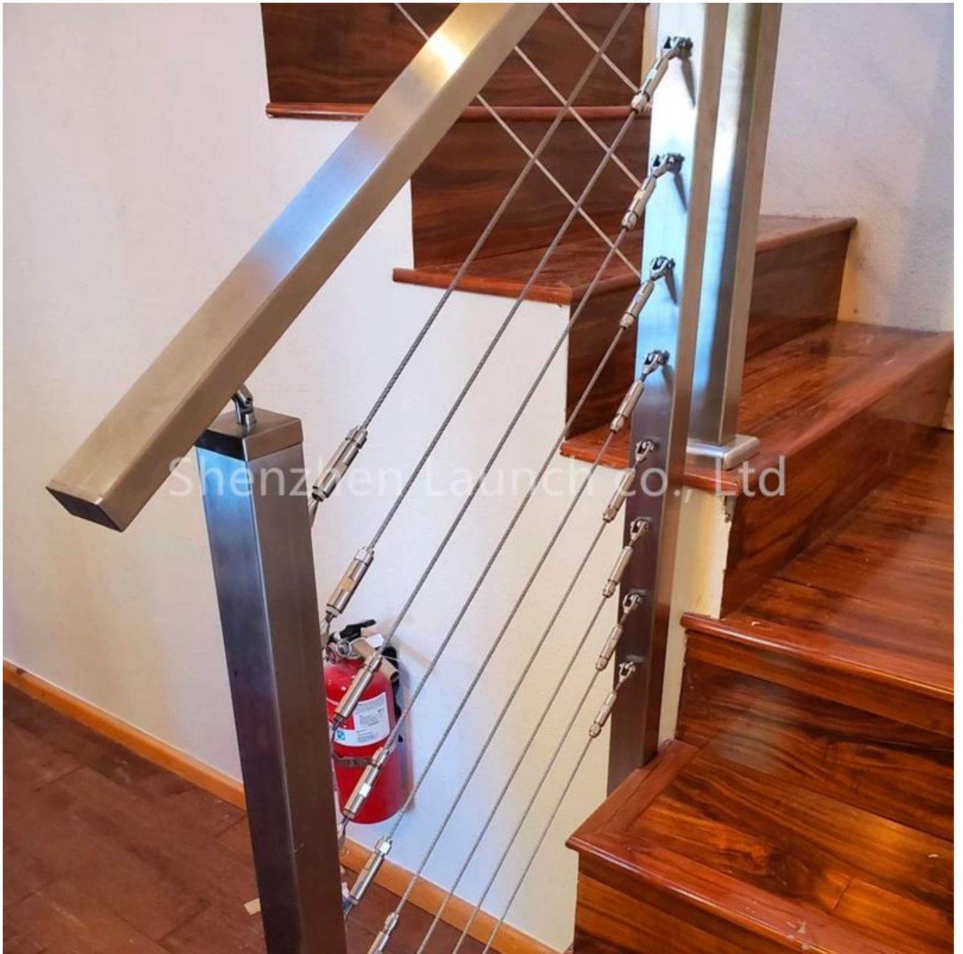
Specs. for T803 swageless wire rope tensioner -
