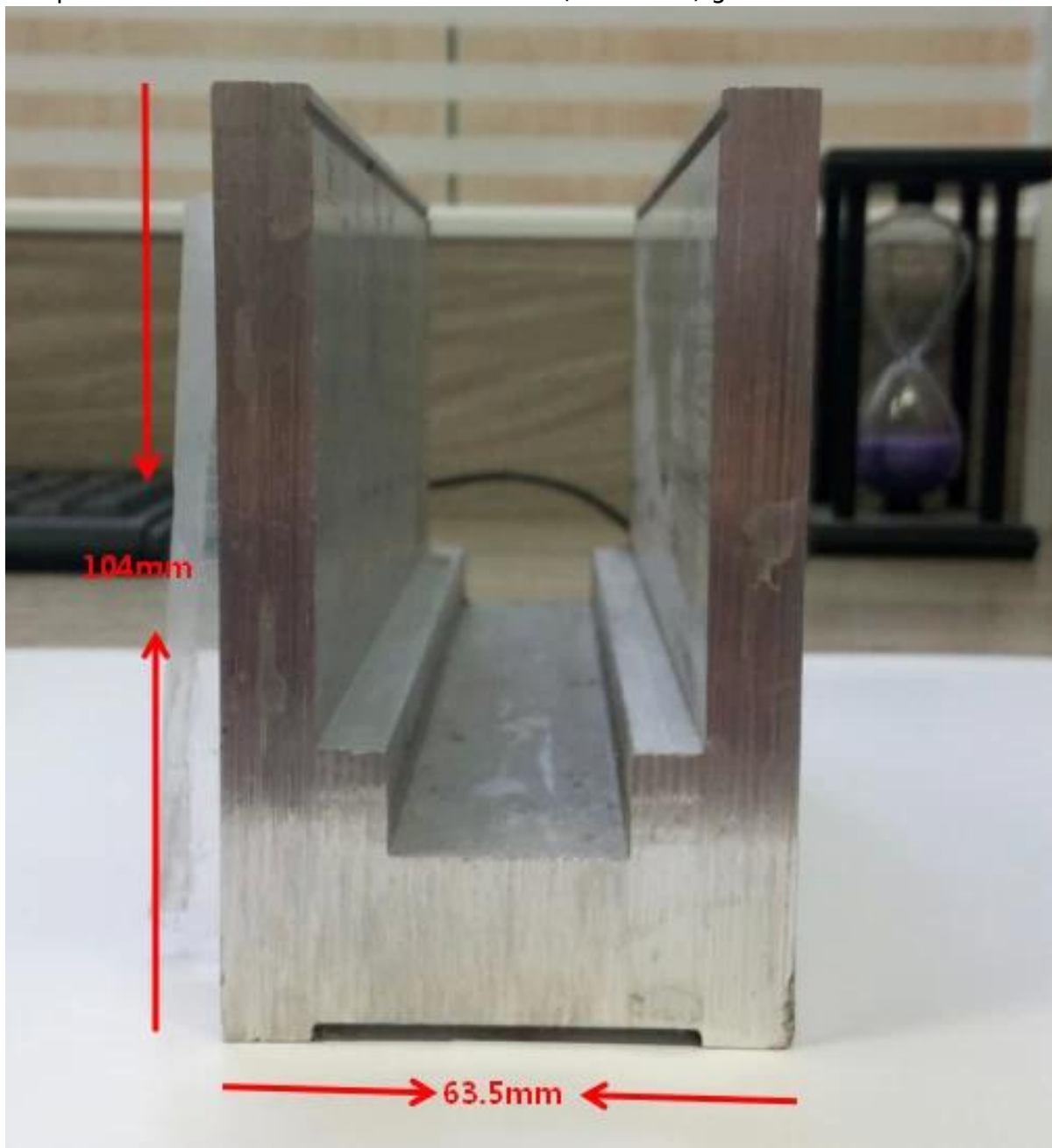
Deep base u-channel for 5/8 inch - 3/4 inch (15-19mm) glass
