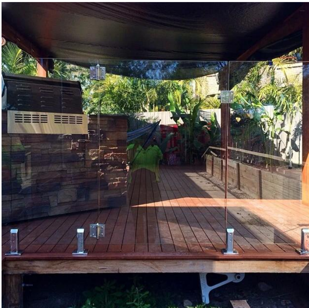
China glass pool fencing, frameless glass fencing spigots
