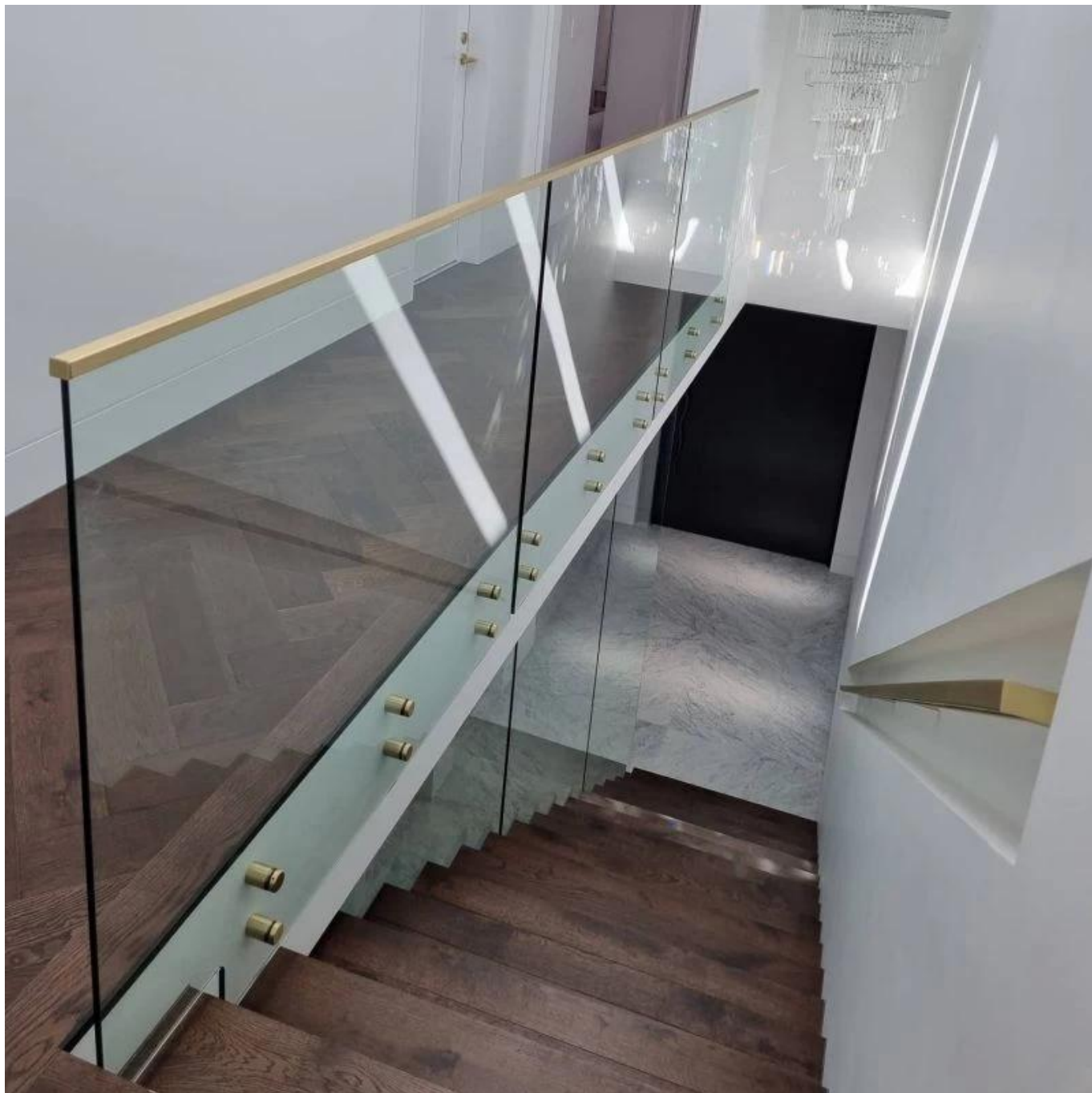
4) Glass standoff + top slotted handrail in black color.
