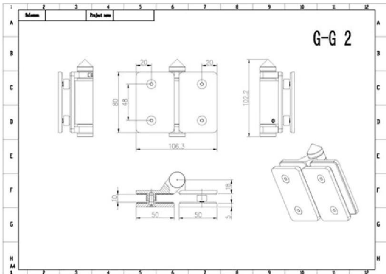
G-G2 glass to glass hinge adjust
