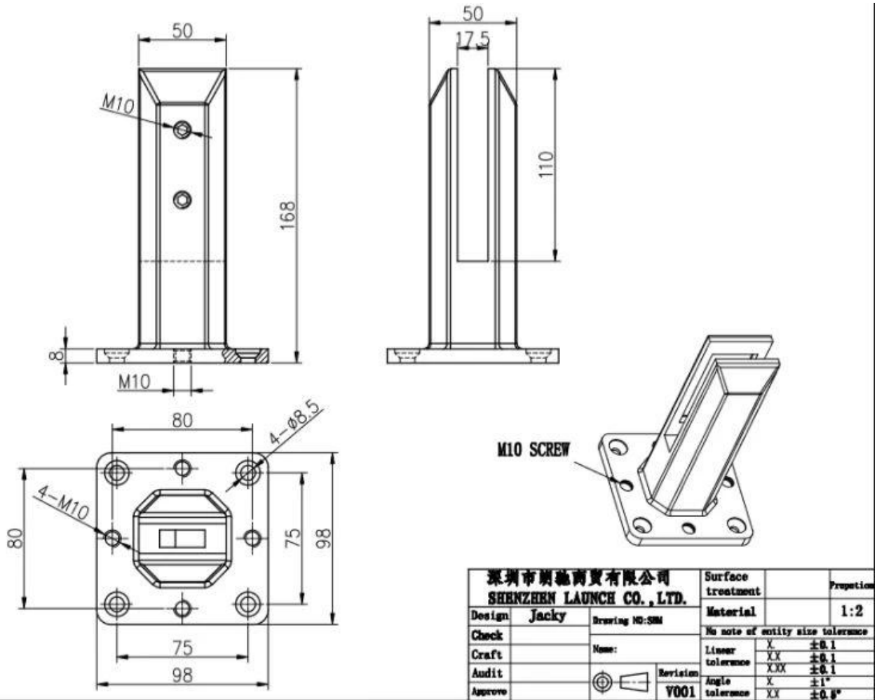
Leveling plate drawing
