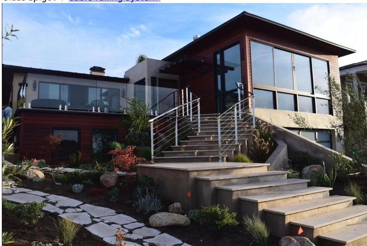
Glass spigot + glass clamp CB-180 + CB-90
