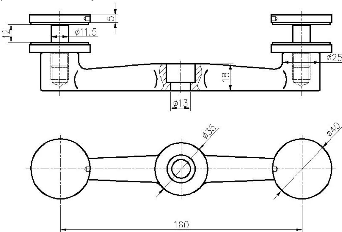
Spider standoff drawing
