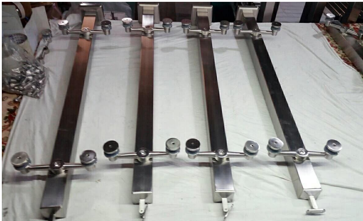
Spider balustrade post with adjustable handrail bracket
