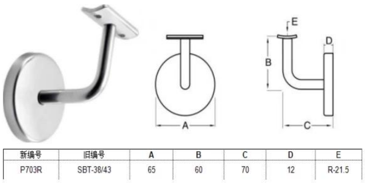
Wall mounted handrail bracket technetical drawing
