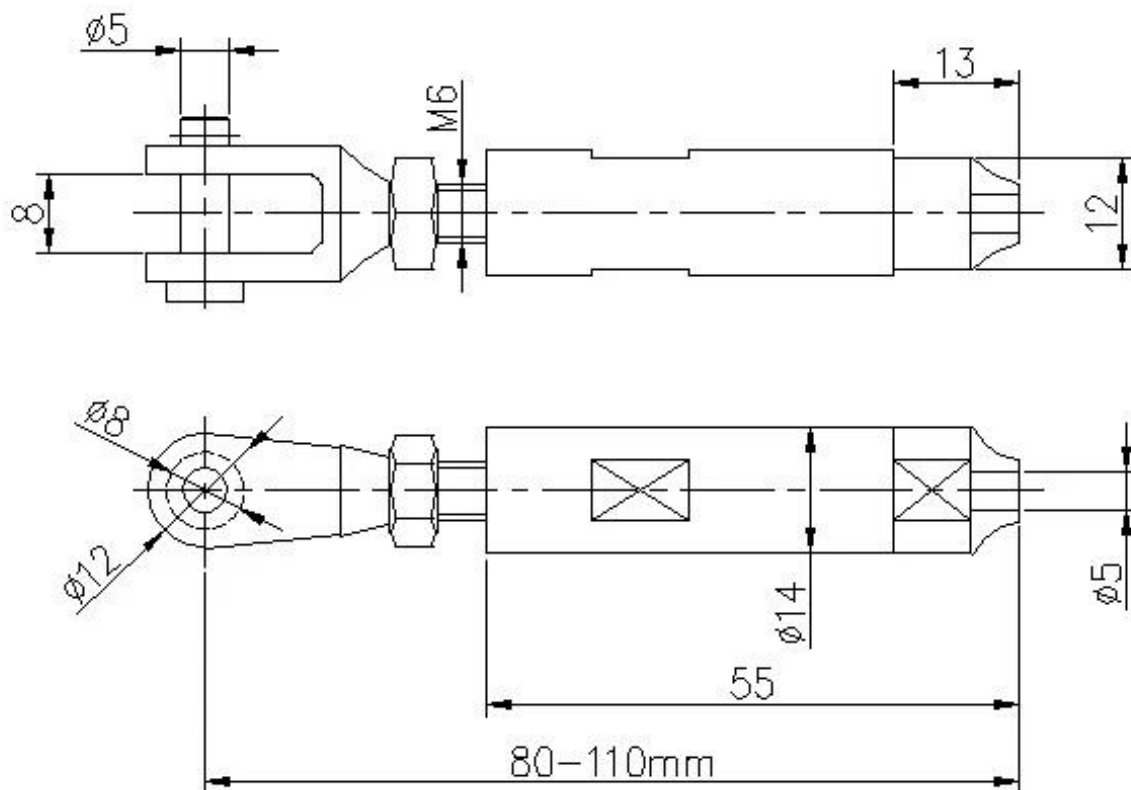
T803 drawing
