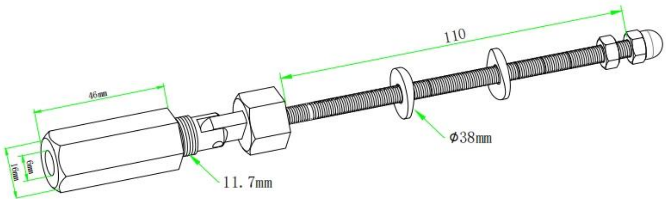
Drawing for small cable tensioner
