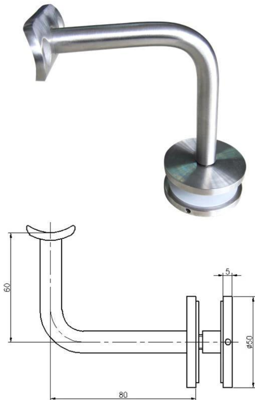
Wall mount handrail bracket model P706
