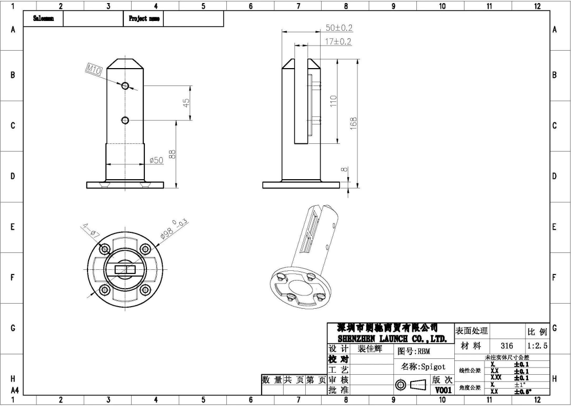
3. square core drill spigot , model # SCM-2
