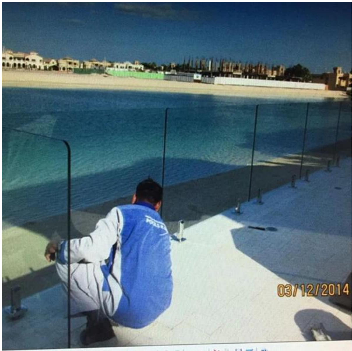
glass spigots for balcony
