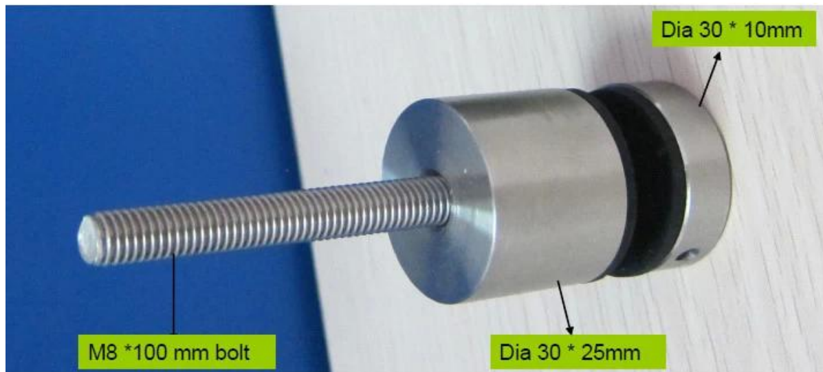
2). Model No. SF-50 glass panel holder standoff.
