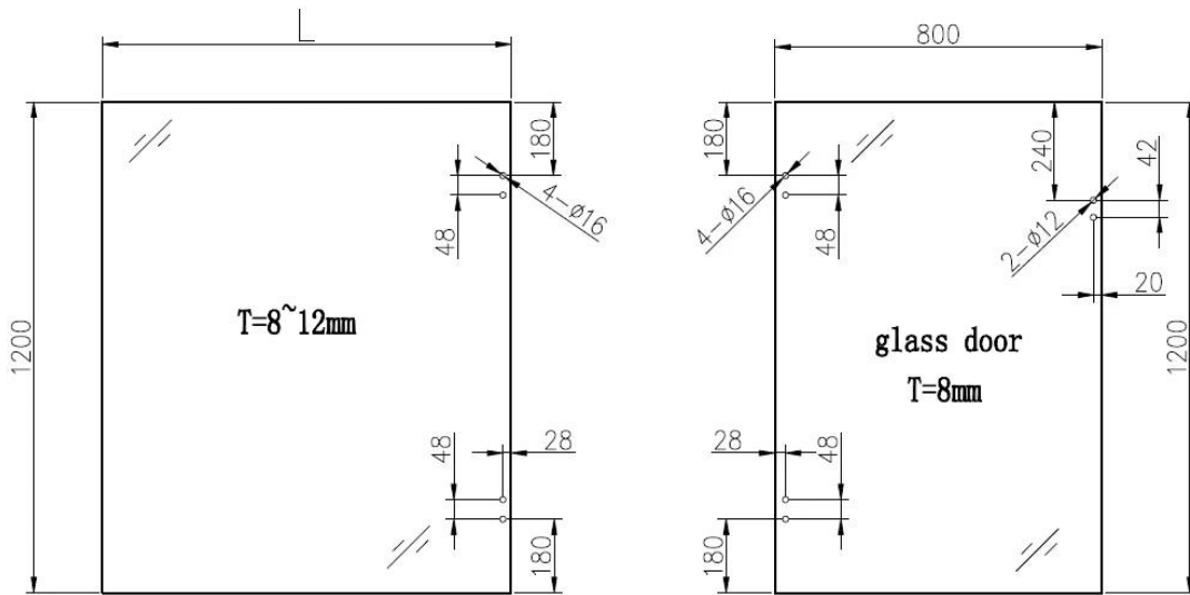
Glass hole location drawing;
