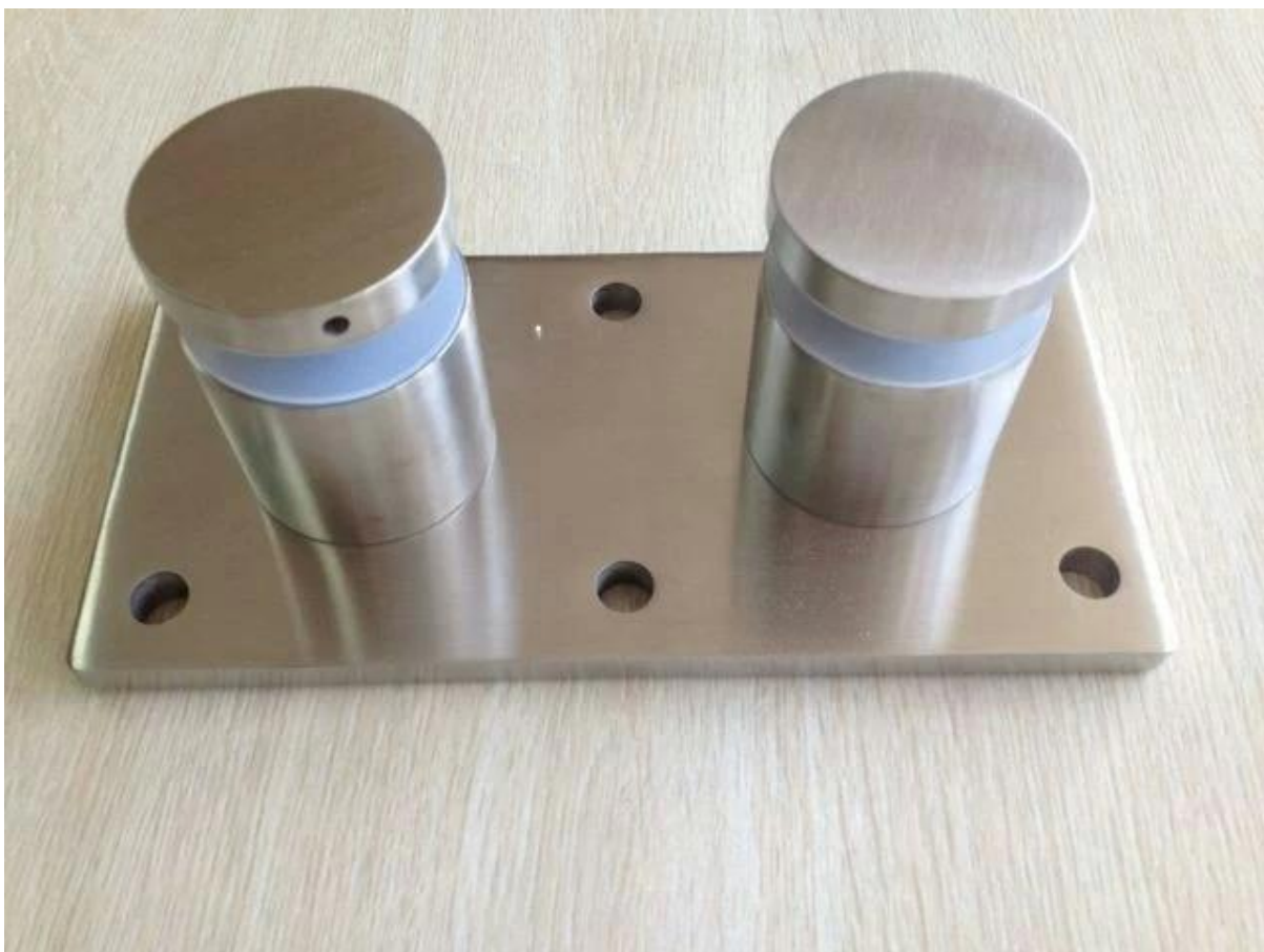
Model No.SF-50T glass standoff
