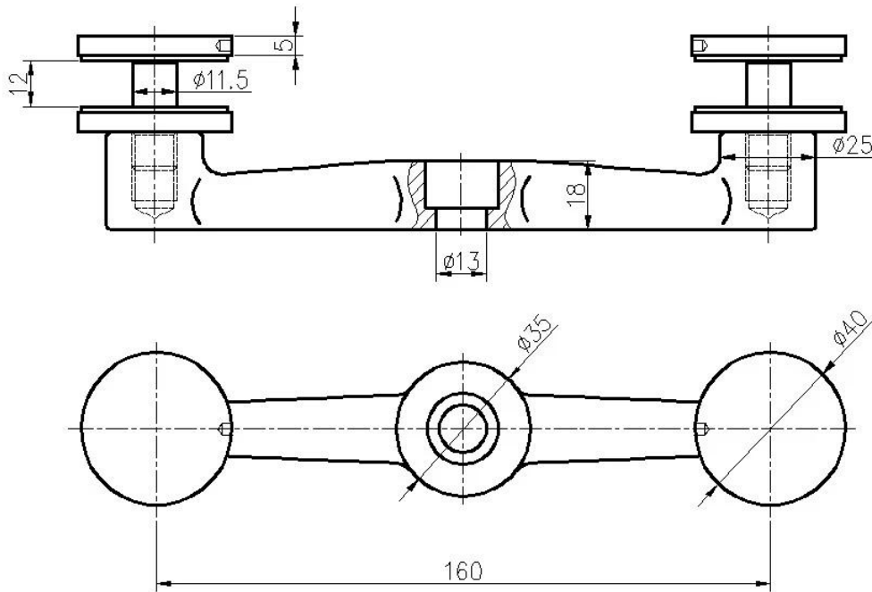
Glass standoff attachment dimensions
